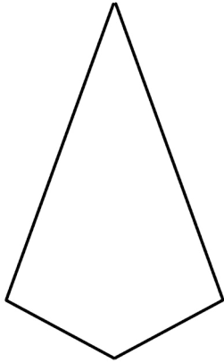
Facet PF-FACE 5.125" h x 3.125" w 17 pc/SF
